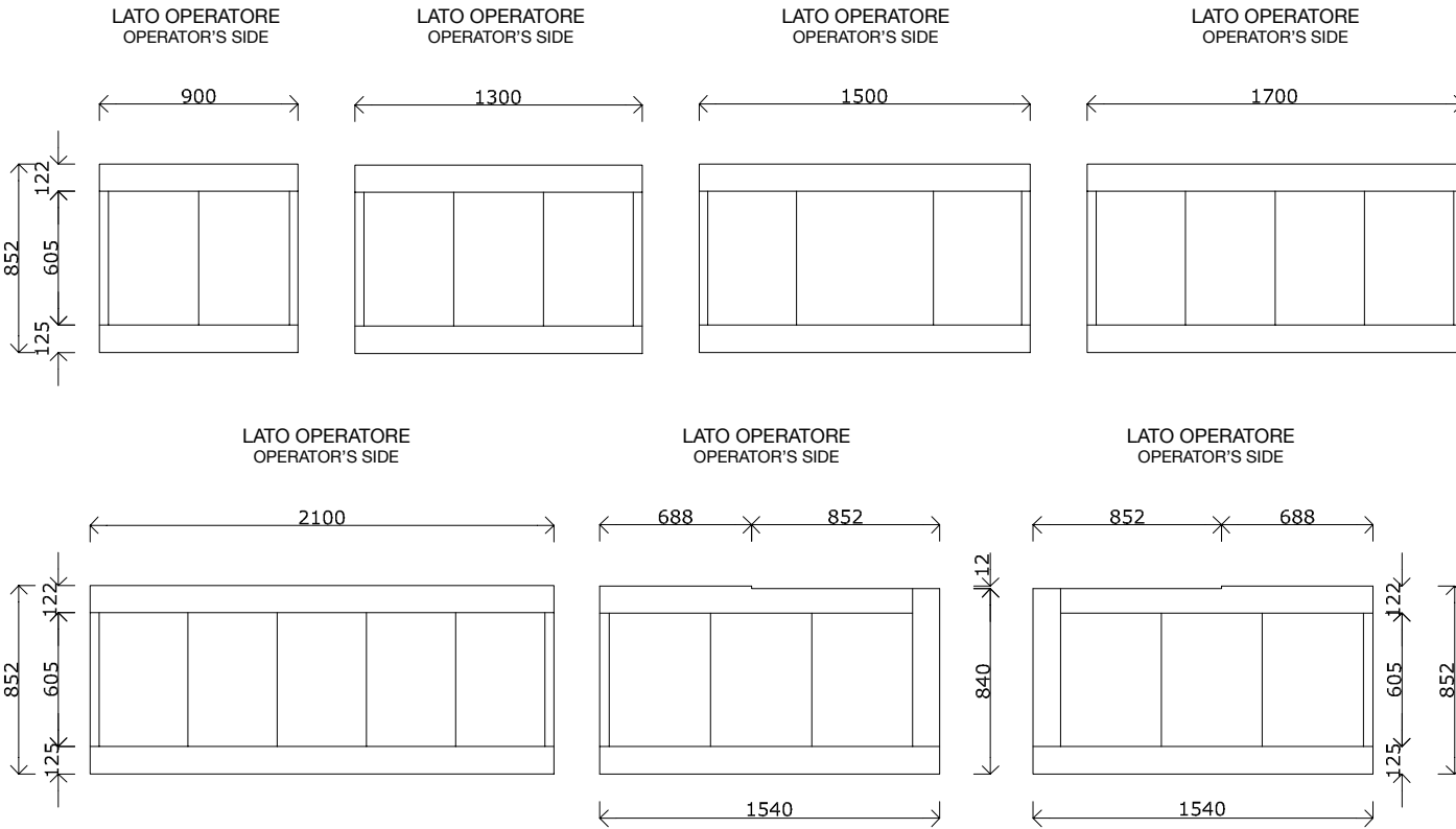
PIANTE / FLOOR DRAWING
