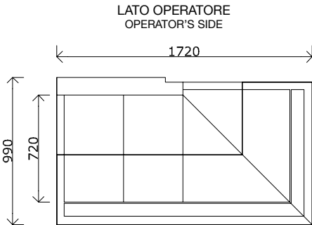
PIANTE / FLOOR DRAWINGS
