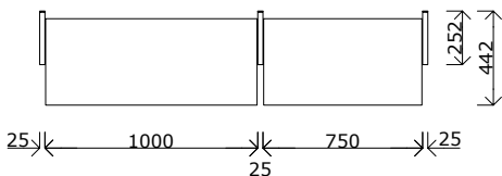
PIANTA / FLOOR DRAWING
