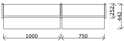
PIANTA / FLOOR DRAWING
