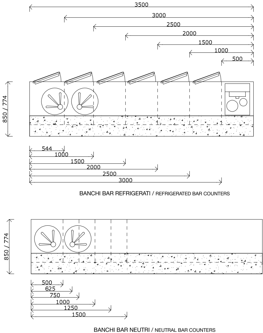
PIANTE/ FLOOR DRAWINGS
